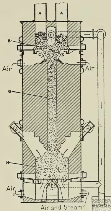
Fig. 80.—Körting Double Zone Up-Draft Gas Producer for Peat.
